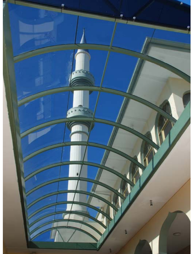
13mm grey laminated annealed curved glass Vaulted glazed roof Auburn Mosque, NSW
